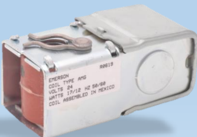
Solenoid Coil
